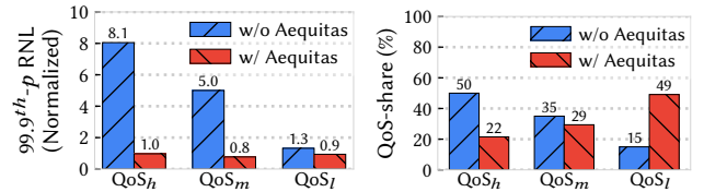
Figure 23: Result from testbed implementation shows that Aequitas maintains SLO compliance and converges to the target QoS-mix.
