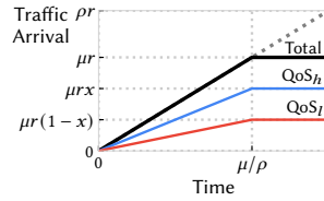
Figure 7: Traffic arrival pattern used in WFQ delay analysis.
