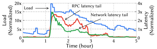
Figure 3: A congestion episode (w/o Aequitas) in production showing that increased load (bits/sec) leads to RPC latency spikes. Higher RNL than RPC latency in some cases is due to sampling differences.
