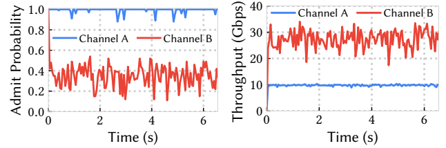
Figure 18: Aequitas maintains a near 1.0 admit probability for in-quota RPC channels that have demand less than fair-share. Excess quota is reclaimed by other channels to provide max-min fairness.
