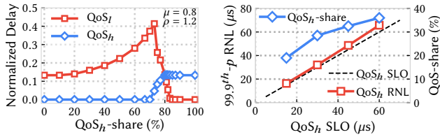
Figure 10: Simulated WFQ compliance: achieved RNL closely tracks SLOs.
