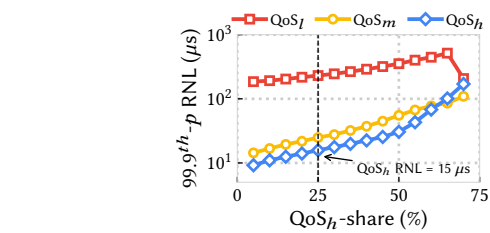
Figure 14: Baseline (w/o Aequitas) 99.9 th -p RNL observed as QoS h -share is varied.
