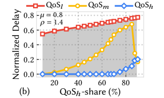
Figure 9: Simulated WFQ worst-case delay with 3 QoS levels under different QoS_h:QoS_m:QoS_I weights: (a) 8:4:1 and (b) 50:4:1. QoS-share of QoS_m and QoS_I is fixed at a ratio of 2:1.
